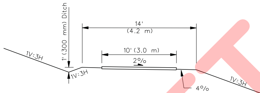
TYPICAL BIKE PATH FOR MINIMAL SHARED USE
