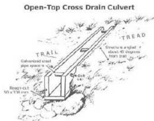
Figure 27--Open-top cross drains or culverts are not
