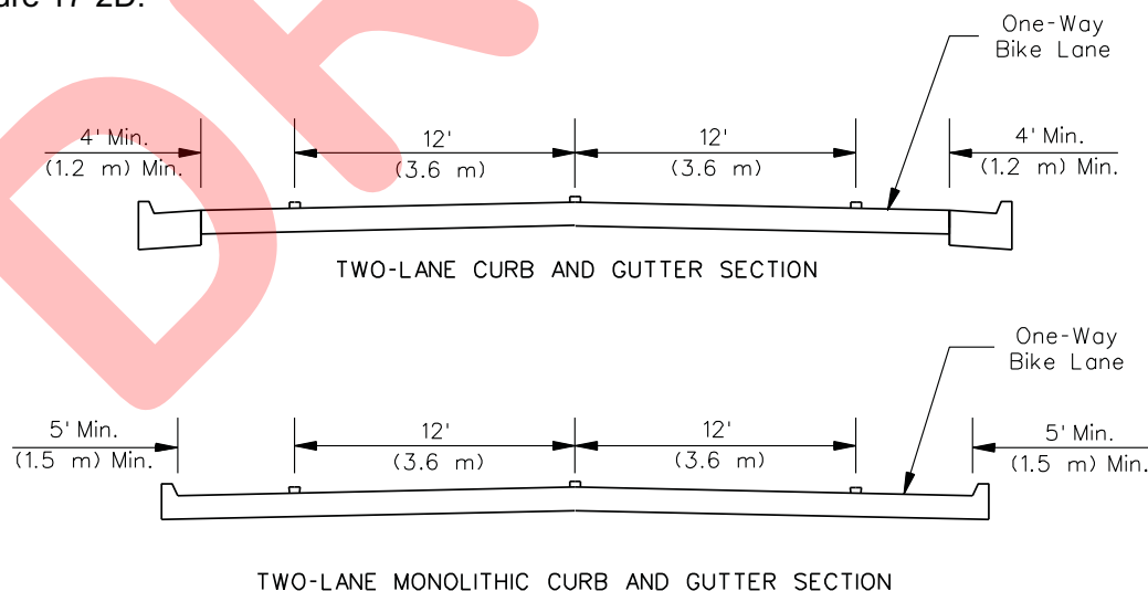
MINIMUM CROSS SECTIONS FOR CURBED STREETS WITHOUT PARKING (Marked Bicycle Lanes)
