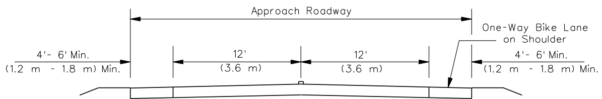
BIKE LANES ON SHOULDERS
