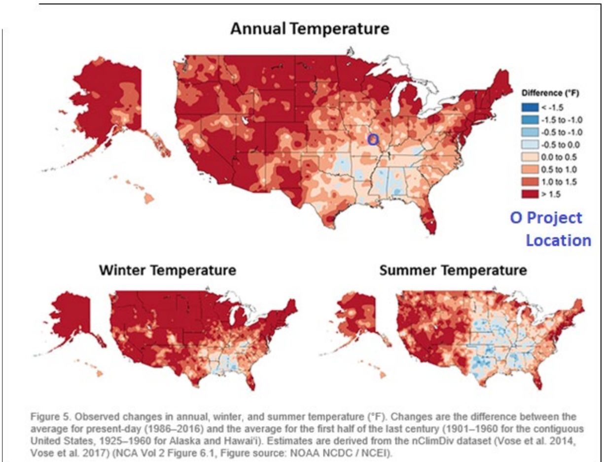
Figure 2. Observed changes in temperature
