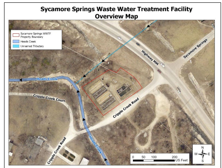
Figure: Sycamore Springs WWTF
