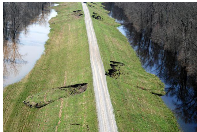
Typical Alton-Gale Levee Slides (2008 Flood)
