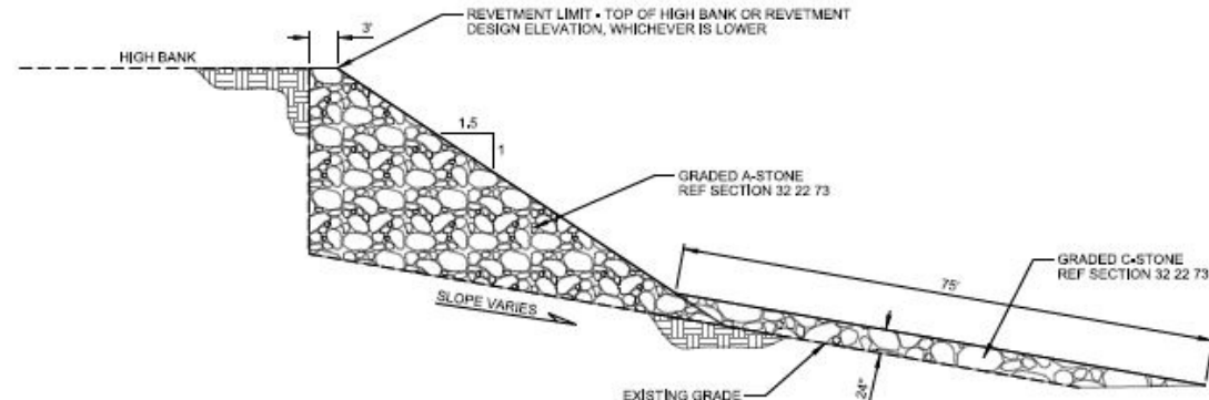
A1 TYPICAL GRADUAL SLOPED REVIEMENT SECTION SCALE: NTS
