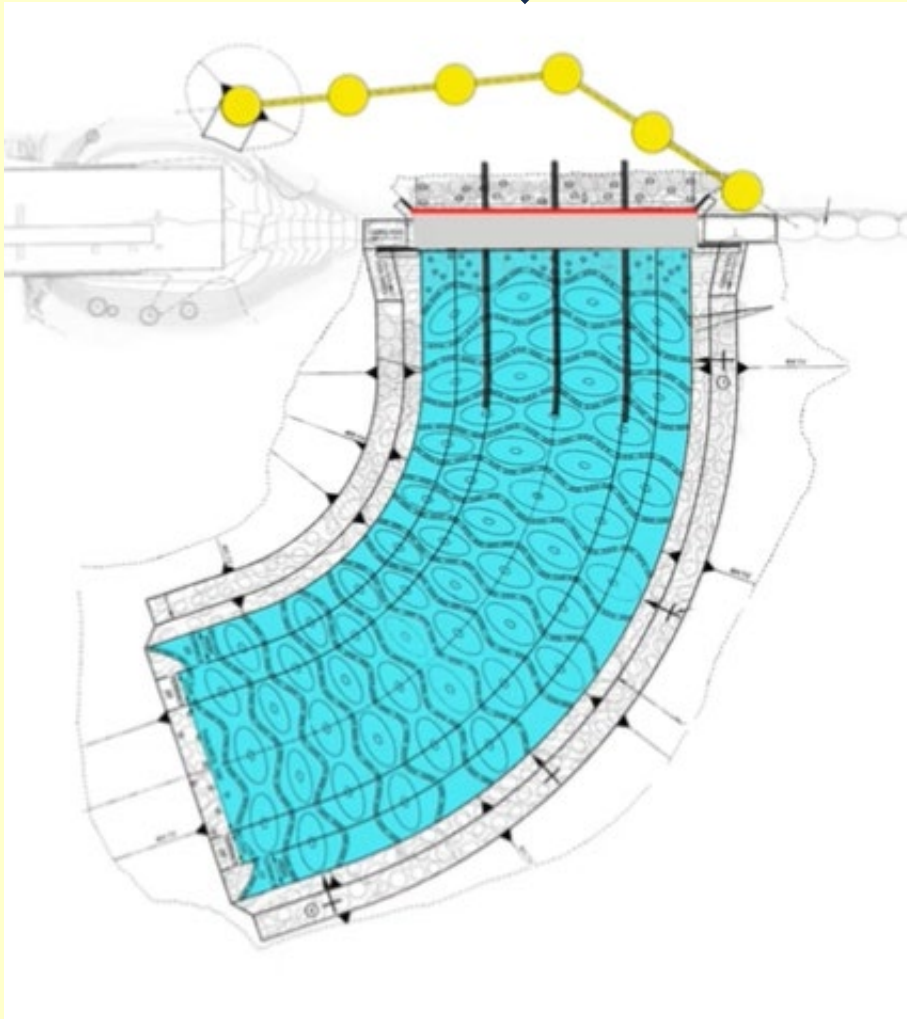
Planned Fish Passage Structure @ 22
