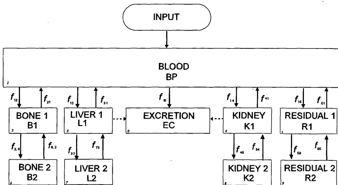
Figure 2-9. Multicompartmental Model
