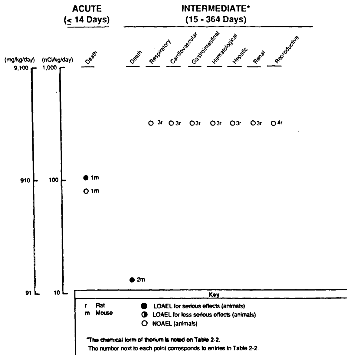
FIGURE 2-2. Levels of Significant Exposure to Thorium - Oral
