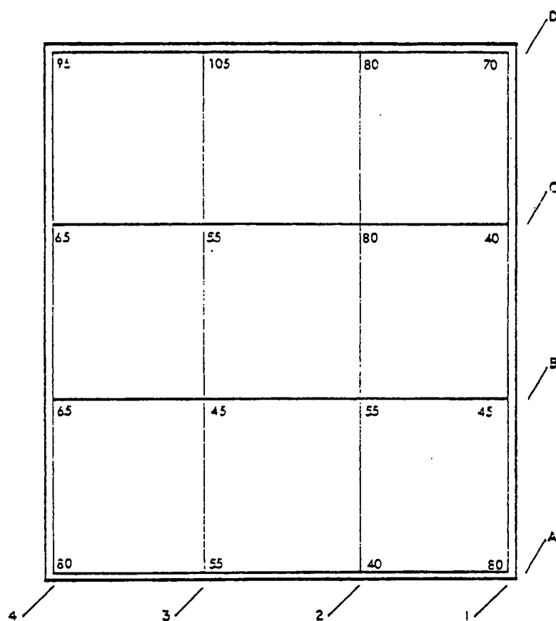
Fig. 9. Building 2: external gamma radiation levels ( \mu\text{R/hr} ) at 1 m above grid points.
