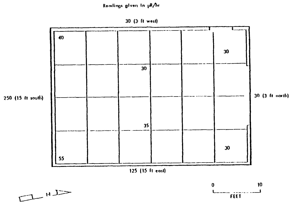
Fig. 12. Building 3, indoors and nearby outdoor points: external gamma levels (in \mu\text{R/hr} ) at 1 m above surface.
