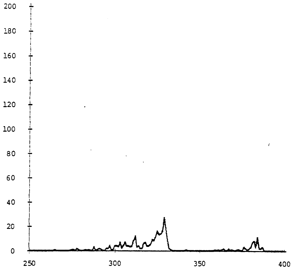
Fig. 25. Alpha spectrum for an air sample taken in Building 2.
