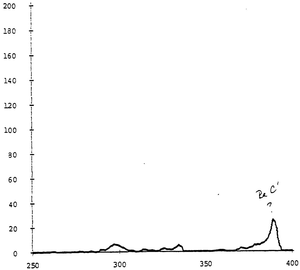
Fig. 25. Alpha spectrum for air sample taken in Building 4.
