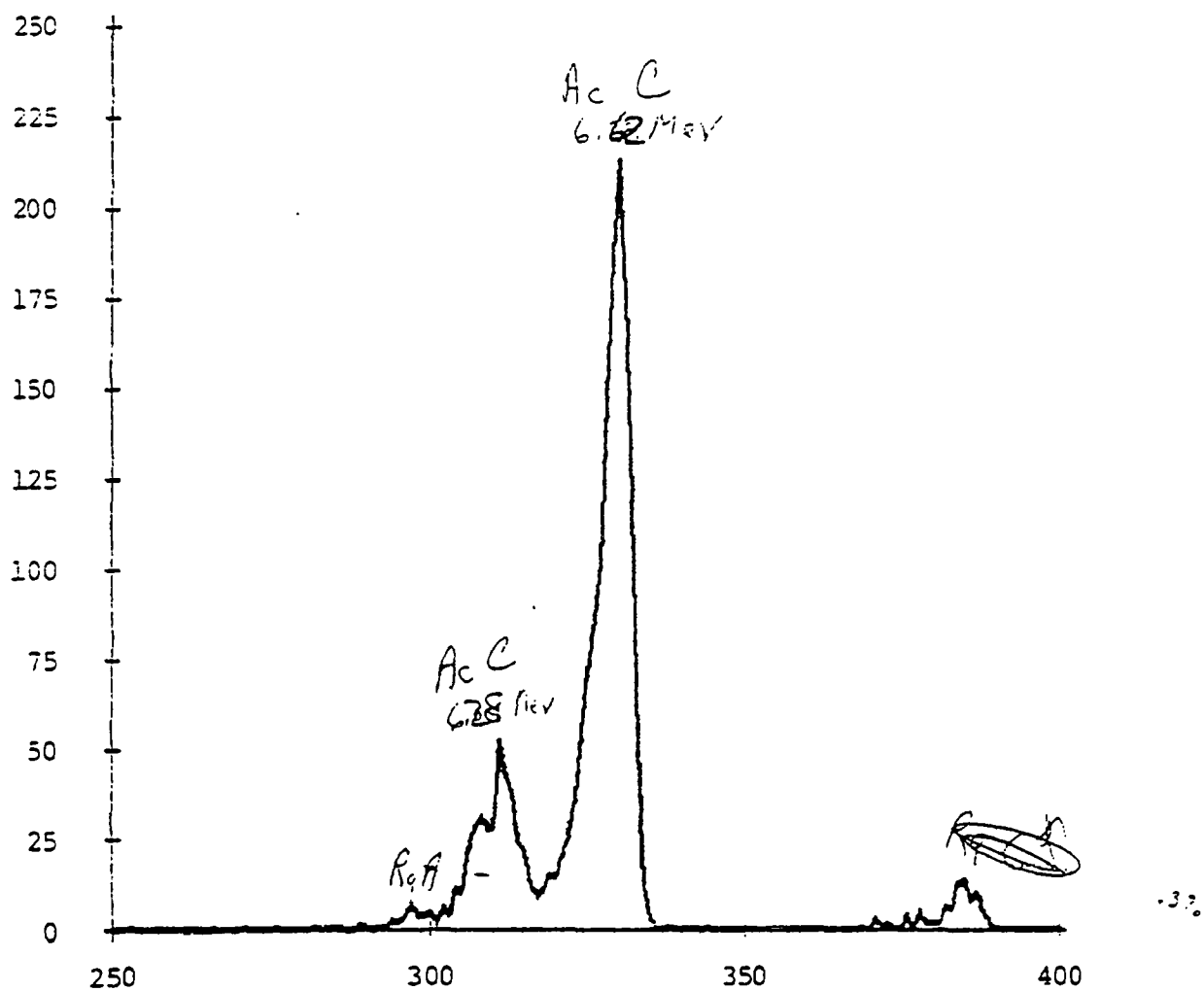
Fig. 22. Alpha spectrum for an air sample taken in Building 1.
