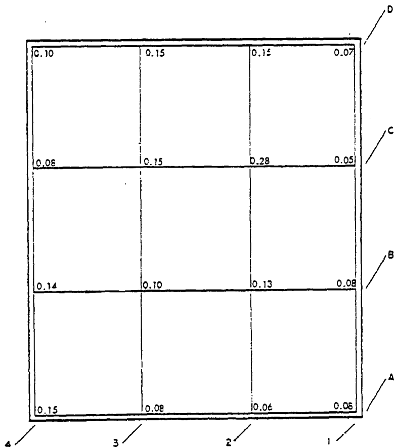
Fig. 7. Building 2, floor: beta-gamma dose rates (mrad/hr) at 1 cm above grid points.
