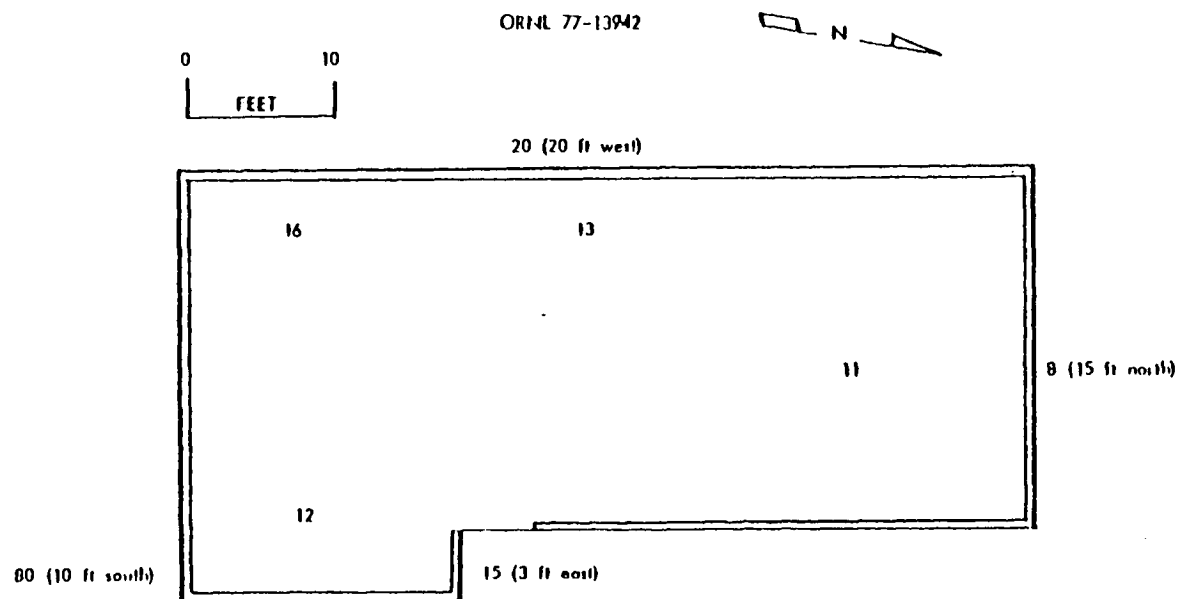
Fig. 14. Building 4, indoors and nearby outdoor points: external gamma radiation levels (in \mu\text{R/hr} ) at 1 m above surface.
