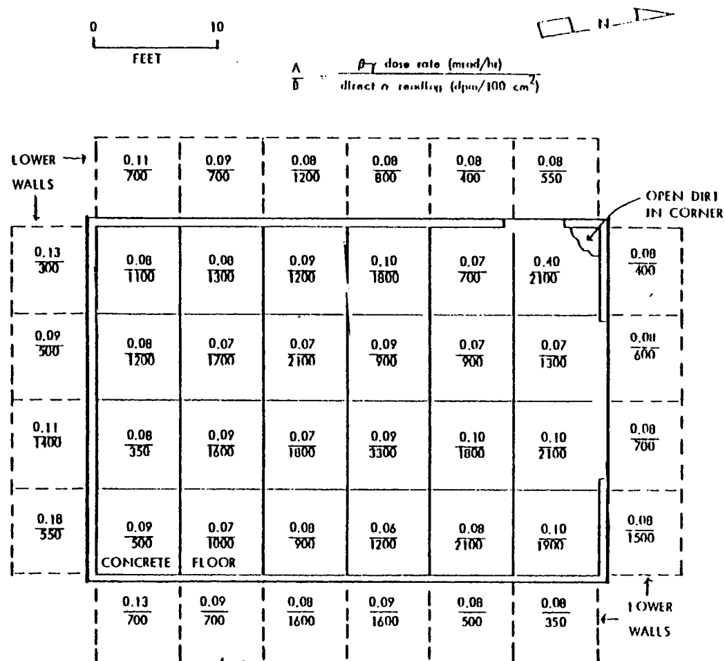
Fig. 11. Building 3, floor and lower walls: maximum observed beta-gamma dose rates and direct alpha measurements.
