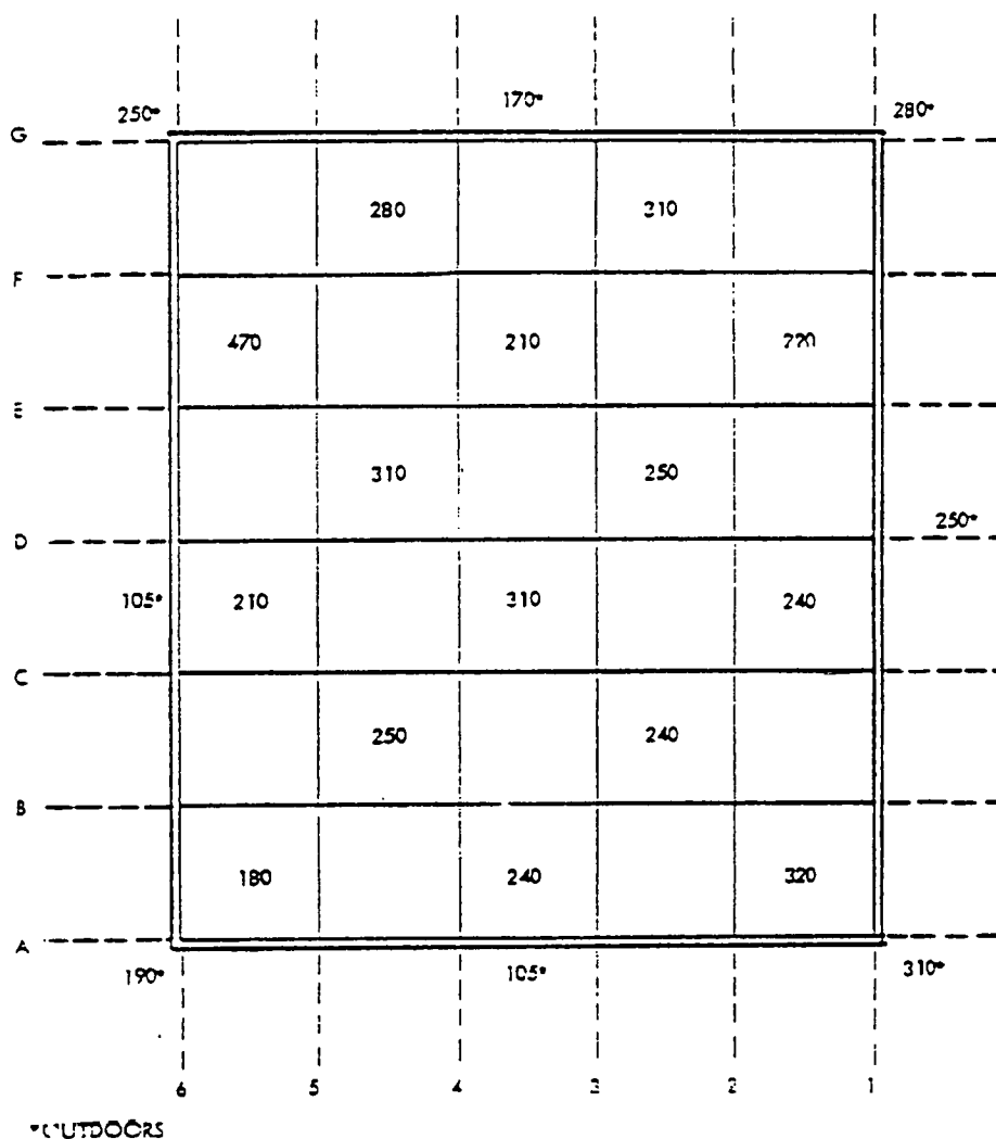
Fig. 6. Building 1; indoors and outdoors within 5 ft of walls; maximum external gamma radiation levels (in uR/hr) within survey blocks, at 1 m above floor.
