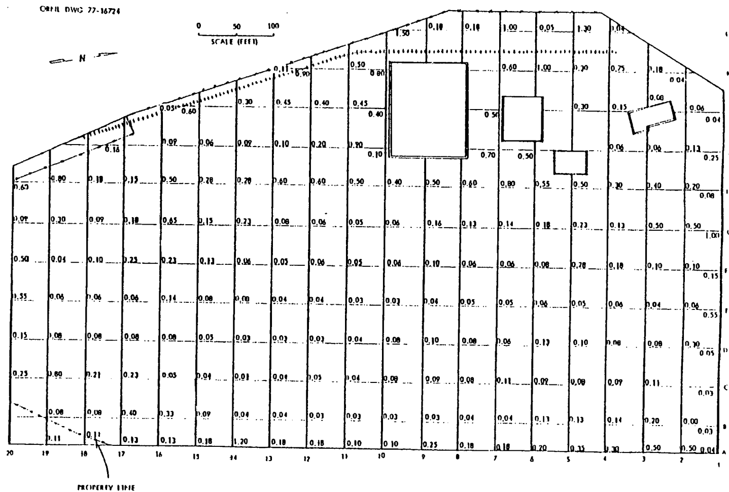
Fig. 17. Beta-gamma dose rates (in mrad/hr) outdoors at 1 cm above grid points.
