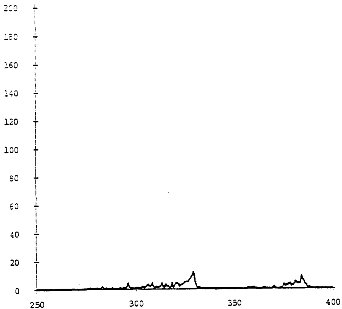
Fig. 24. Alpha spectrum for air sample taken in Building 3.
