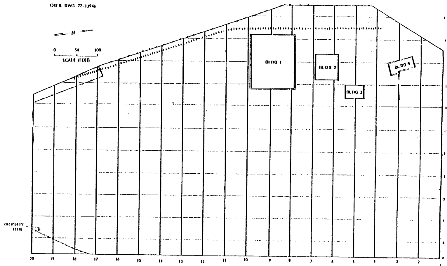
Fig. 1. Scaled drawing of the site and grid used for outdoor survey.
