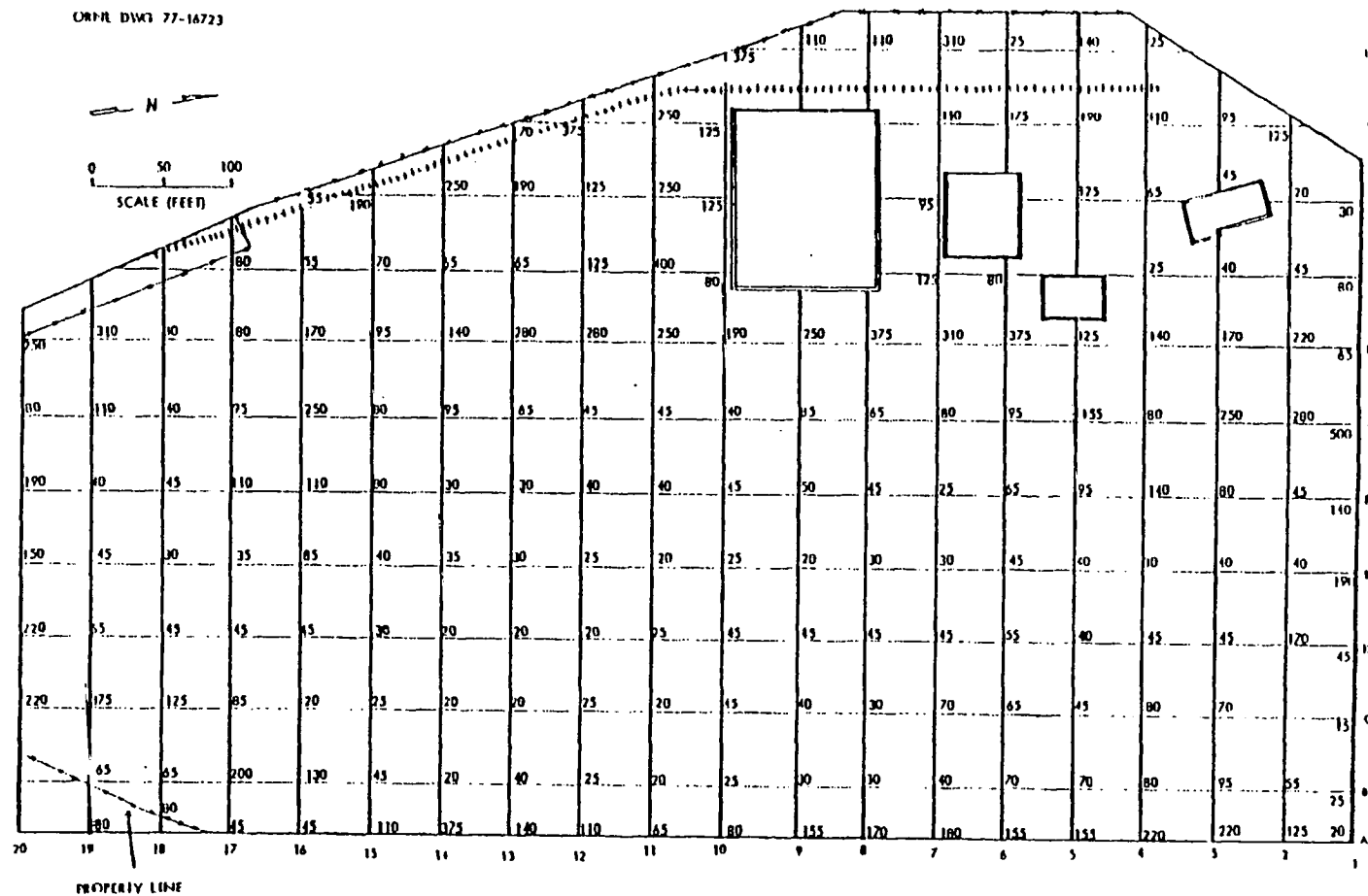
Fig. 19. External gamma radiation levels (in \mu\text{R/hr} ) outdoors at 1 m above grid points.
