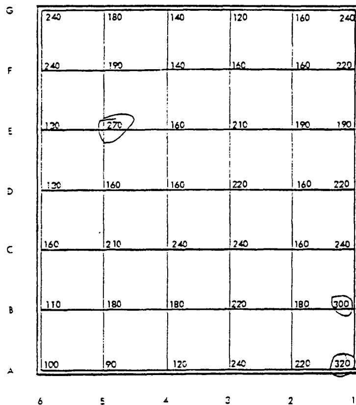
Fig. 3. Building 1, external gamma radiation levels (in \mu\text{R/hr} ) at 1 m above grid points.
