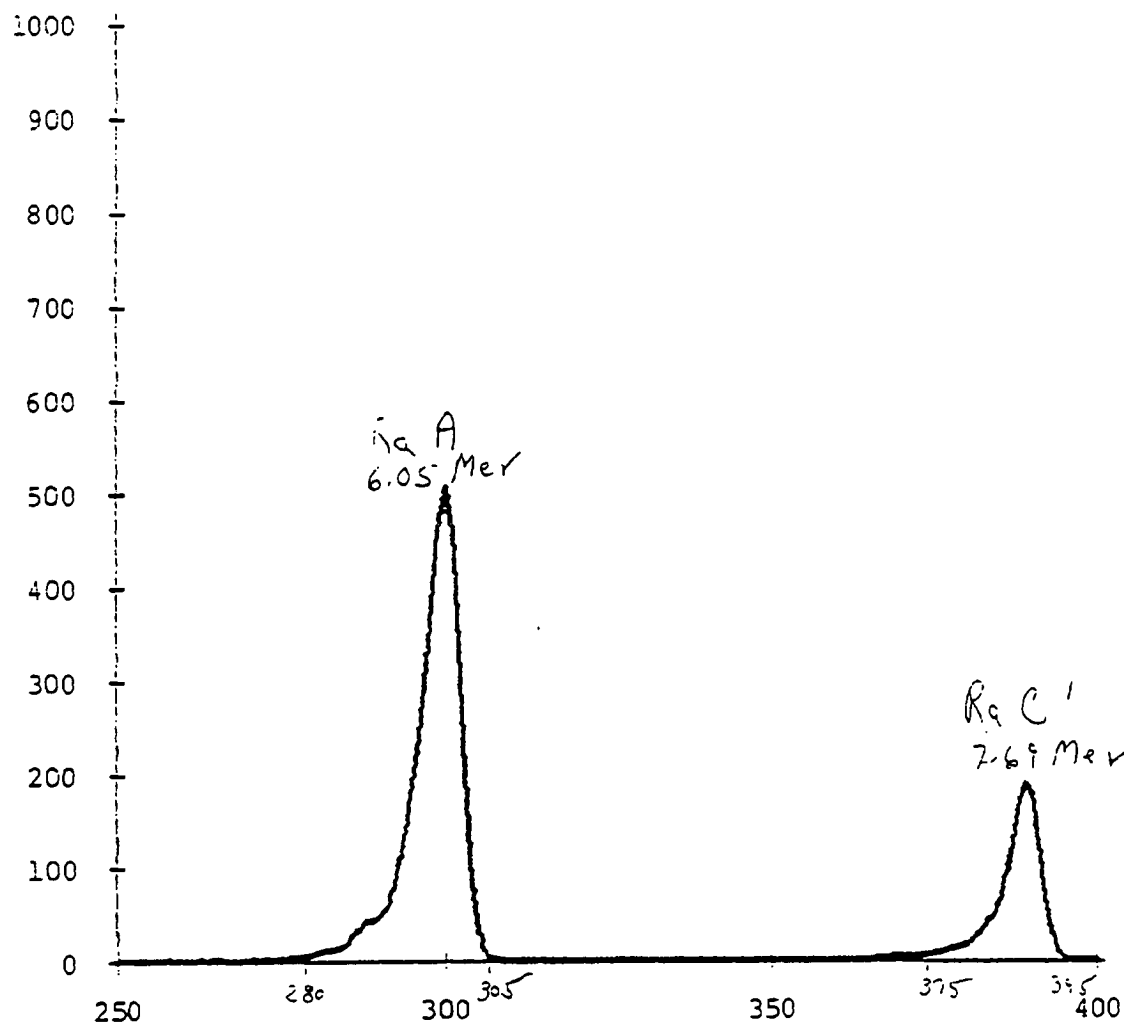
Fig. 21. A typical ^{222}\text{Rn} daughter alpha spectrum.
