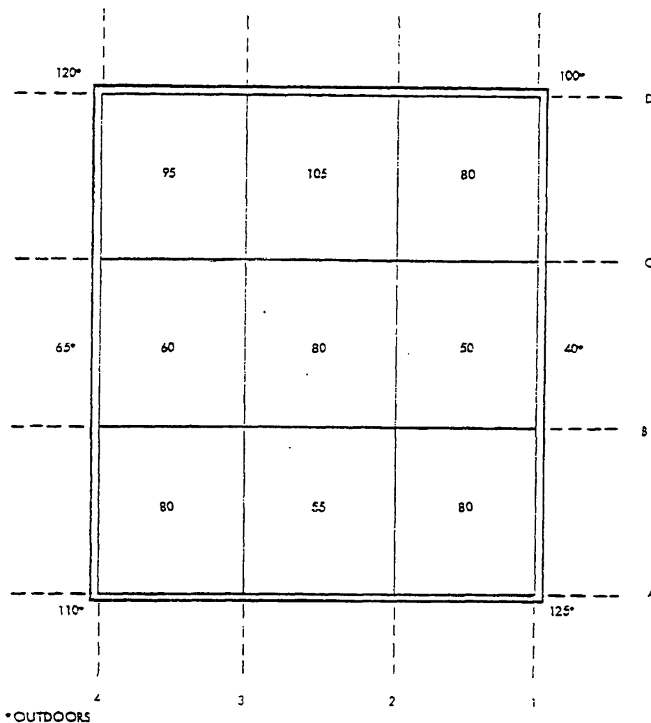
Fig. 10. Building 2, indoors and outdoors within 5 ft of walls: maximum external gamma radiation levels (in \mu\text{R/hr} ) within survey blocks, at 1 m above floor.
