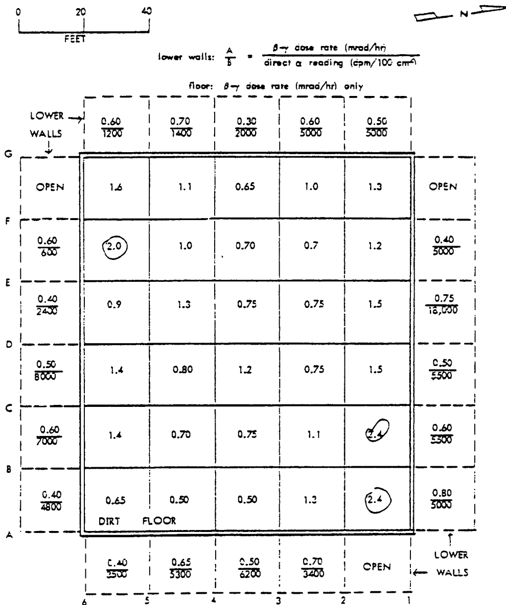
Fig. 4. Building 1, floor and lower walls: maximum observed beta-gamma dose rates and direct alpha readings.
