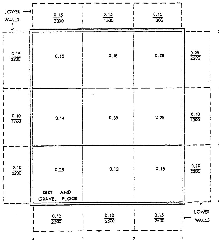
Fig. 8. Building 2, floor and lower walls: maximum observed beta-gamma dose rates and direct alpha readings.
