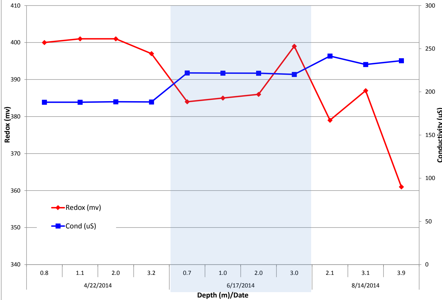
WAP-6 Redox & Conductivity vs Depth
