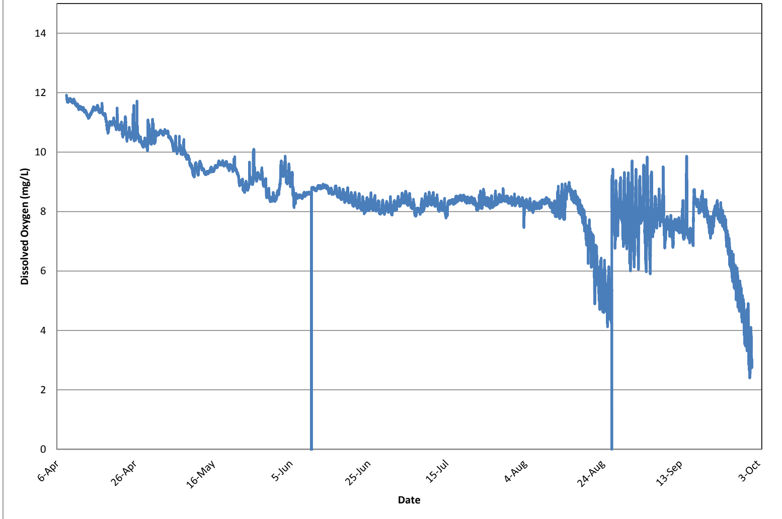
Dissolved Oxygen in spillway as monitored by remote sonde
