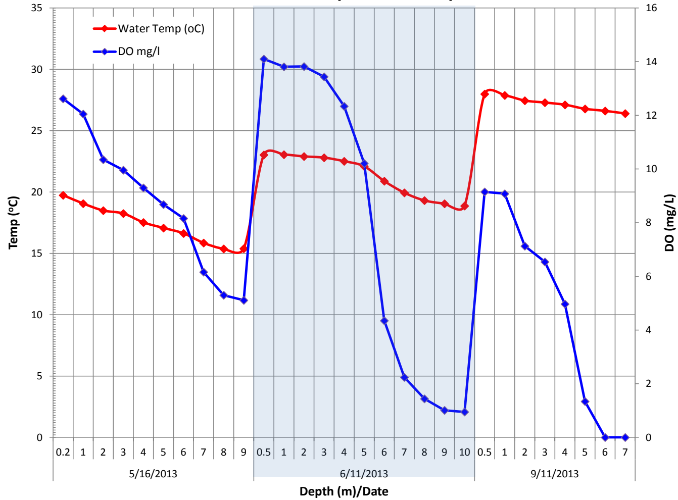
SBV-11 Temp & DO vs Depth
