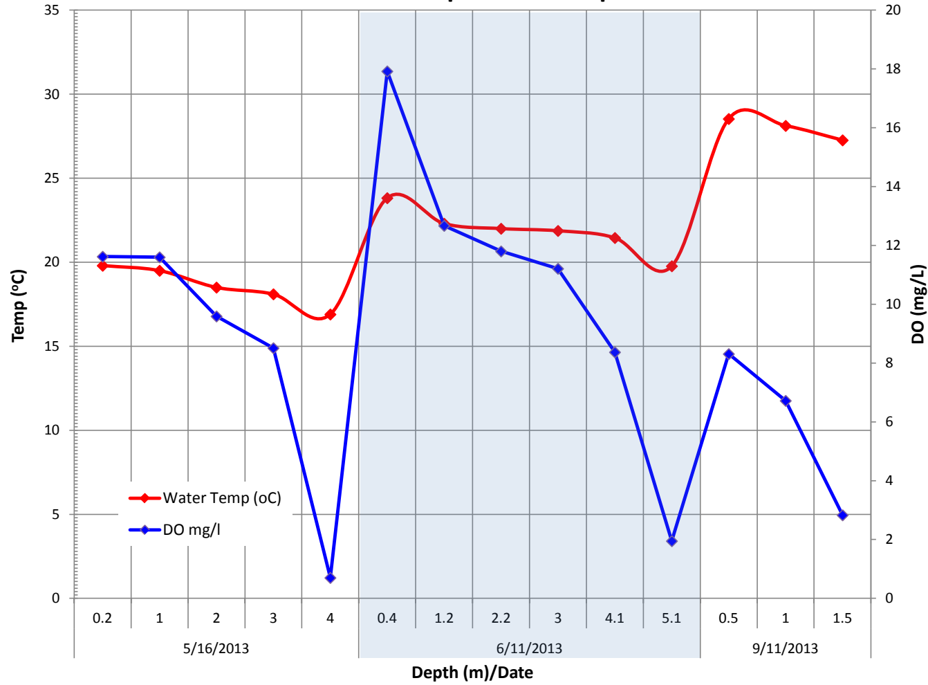
SBV-4 Temp & DO vs Depth
