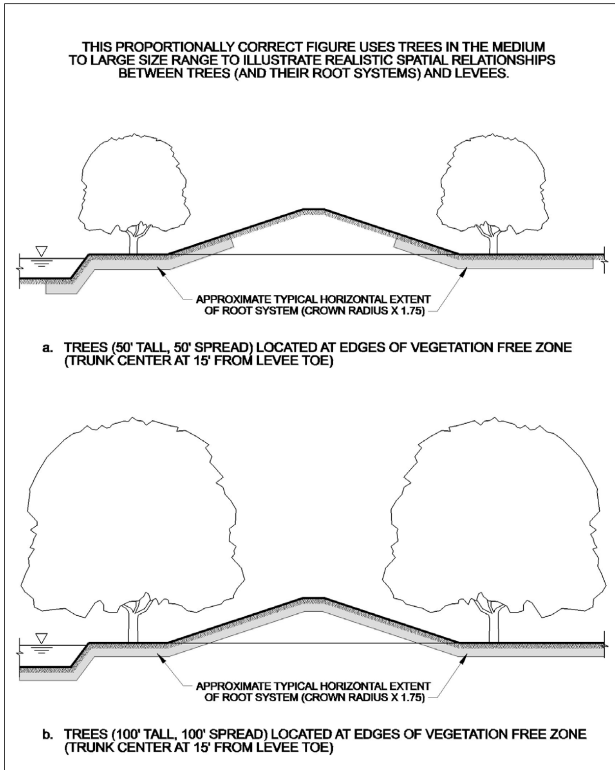
Figure A-24. Levee (20 ft tall, 3:1 side slopes) with Trees, as Noted Above.
