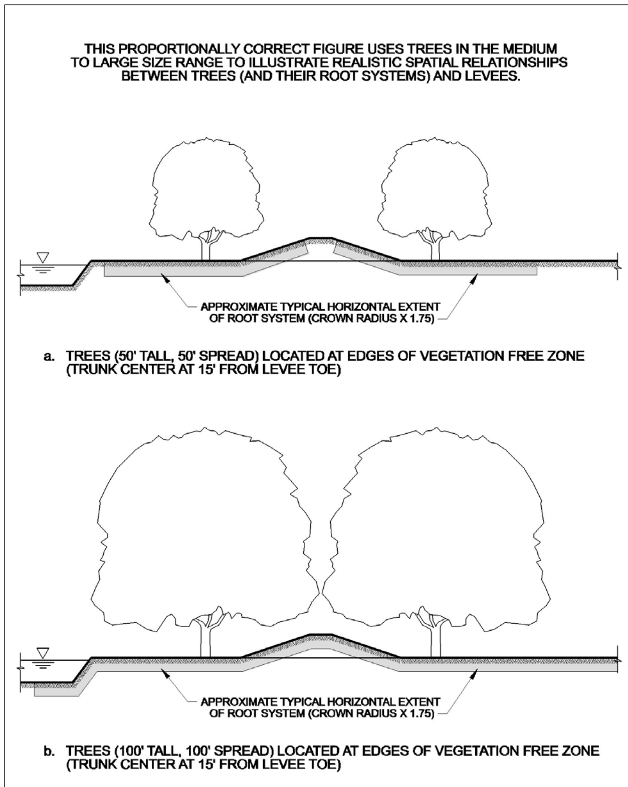
Figure A-25. Levee (10 ft tall, 3:1 side slopes) with Trees, as Noted Above.
