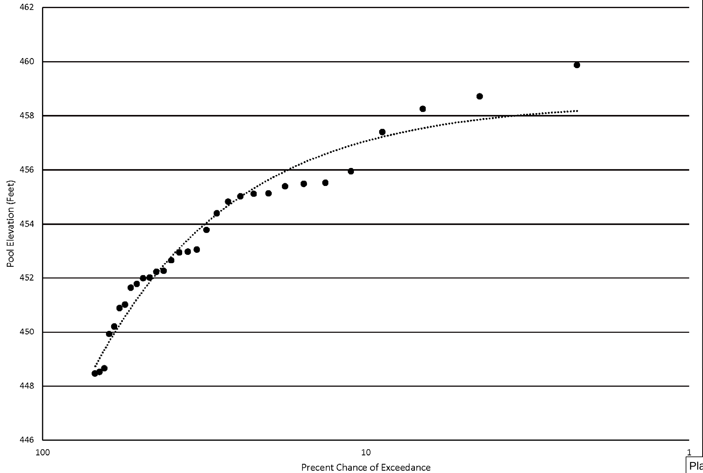
Carlyle Lake - Frequency Curve (1975-2016)
