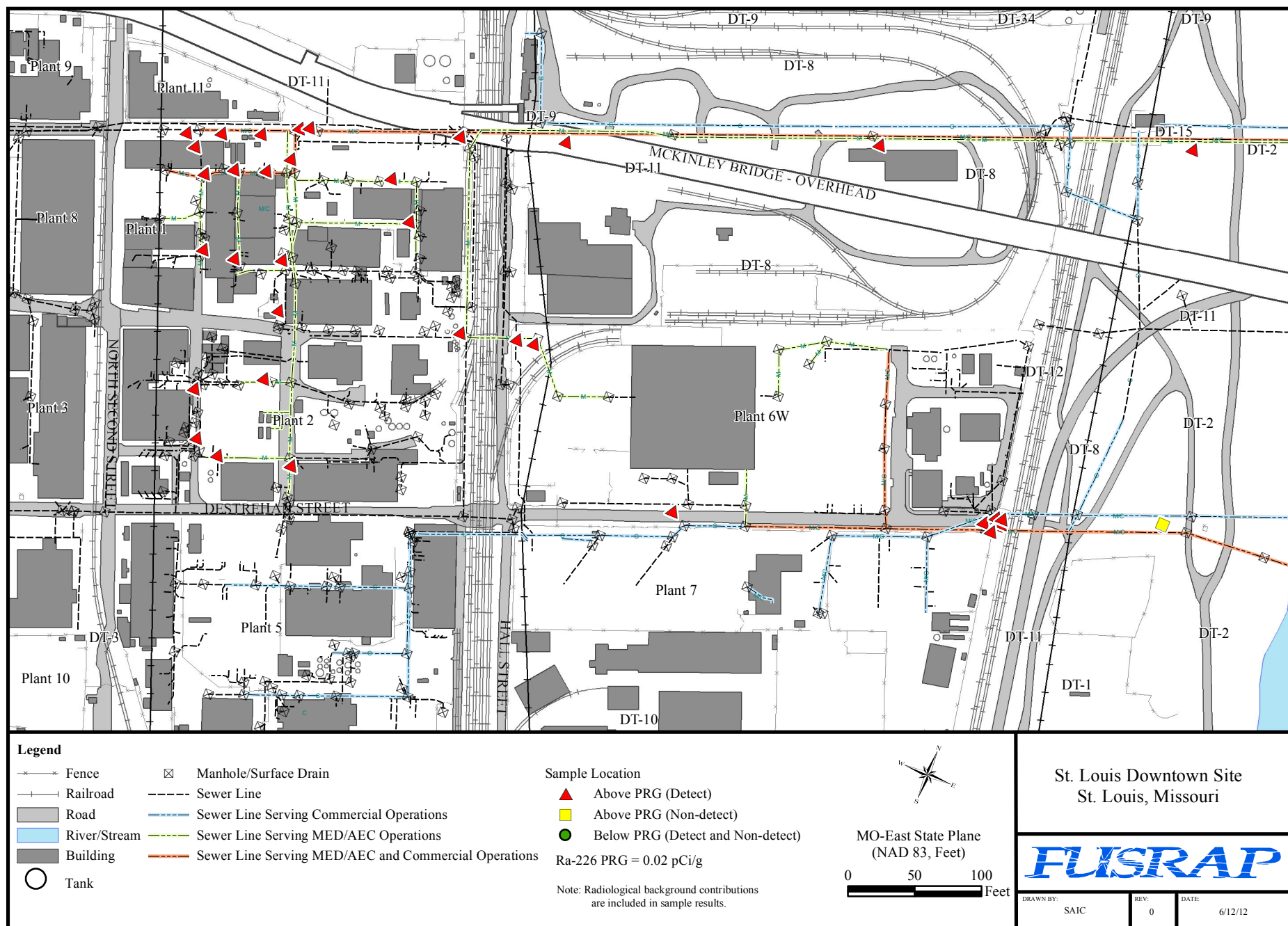
Figure H-24. Distribution of Ra-226 Exceeding the PRG in Soil Adjacent to Sewers
