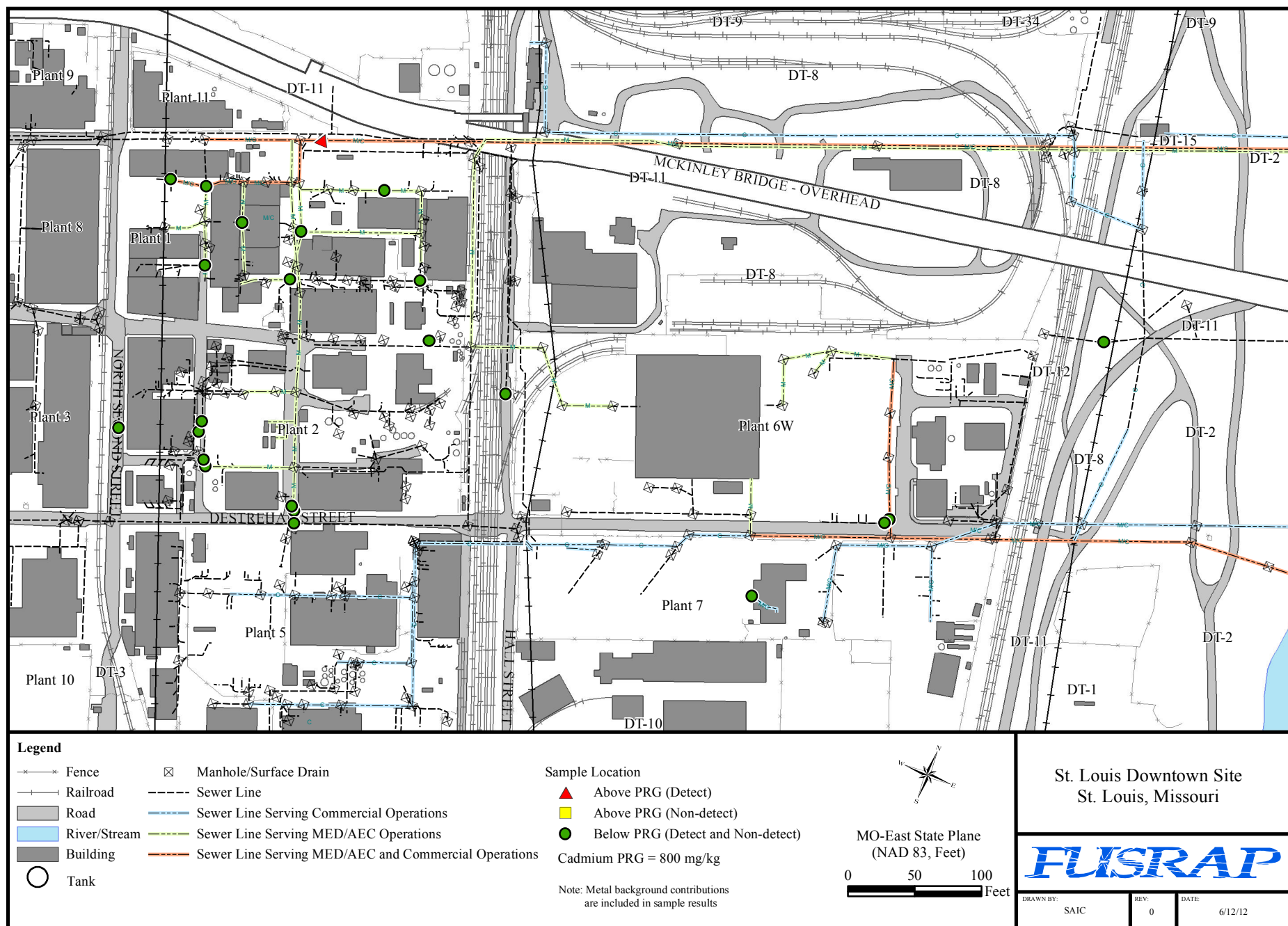
Figure H-11. Distribution of Cadmium Exceeding the PRG in Sewer Sediment
