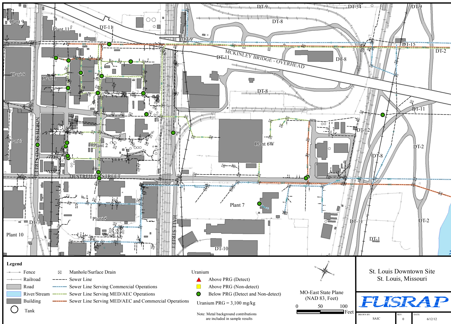
Figure H-19. Distribution of Uranium Metal Exceeding the PRG in Sewer Sediment
