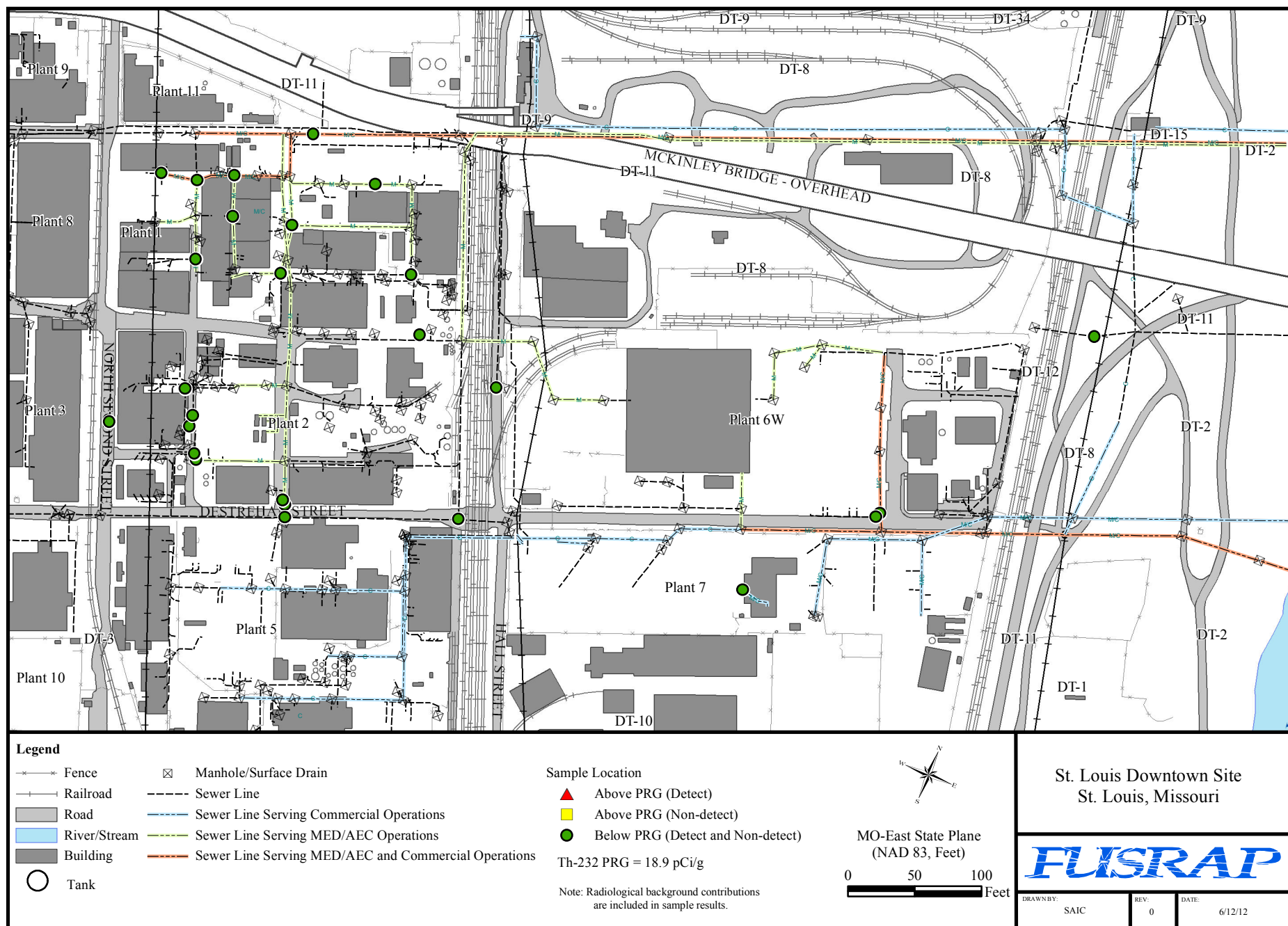
Figure H-7. Distribution of Th-232 Exceeding the PRG in Sewer Sediment
