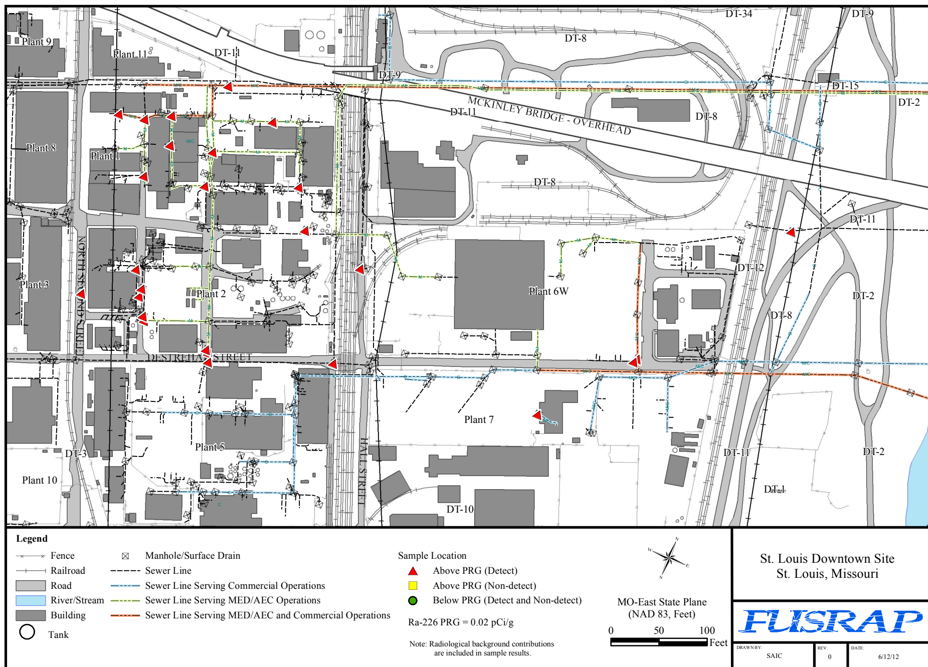
Figure H-3. Distribution of Ra-226 Exceeding the PRG in Sewer Sediment
