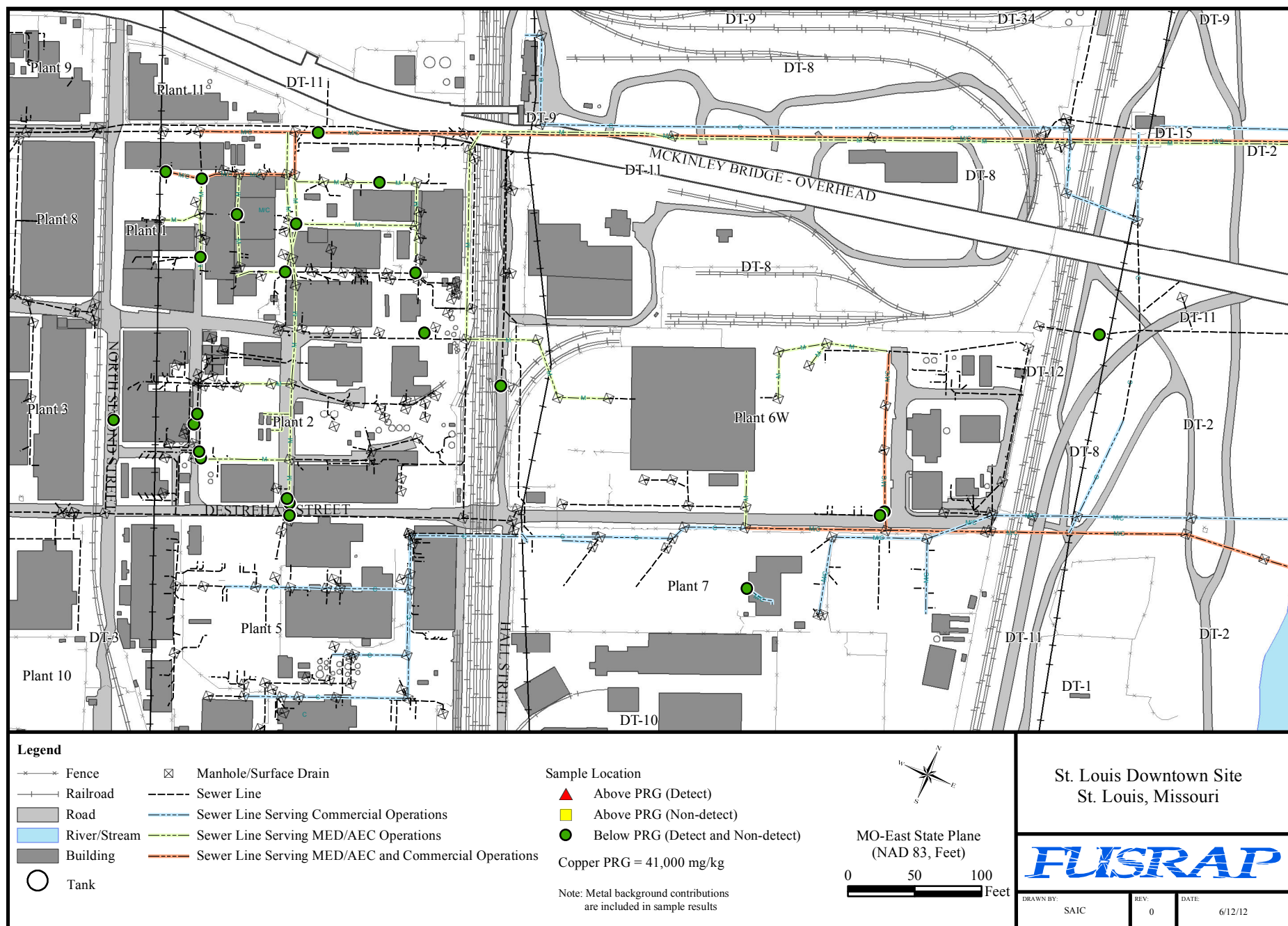
Figure H-13. Distribution of Copper Exceeding the PRG in Sewer Sediment
