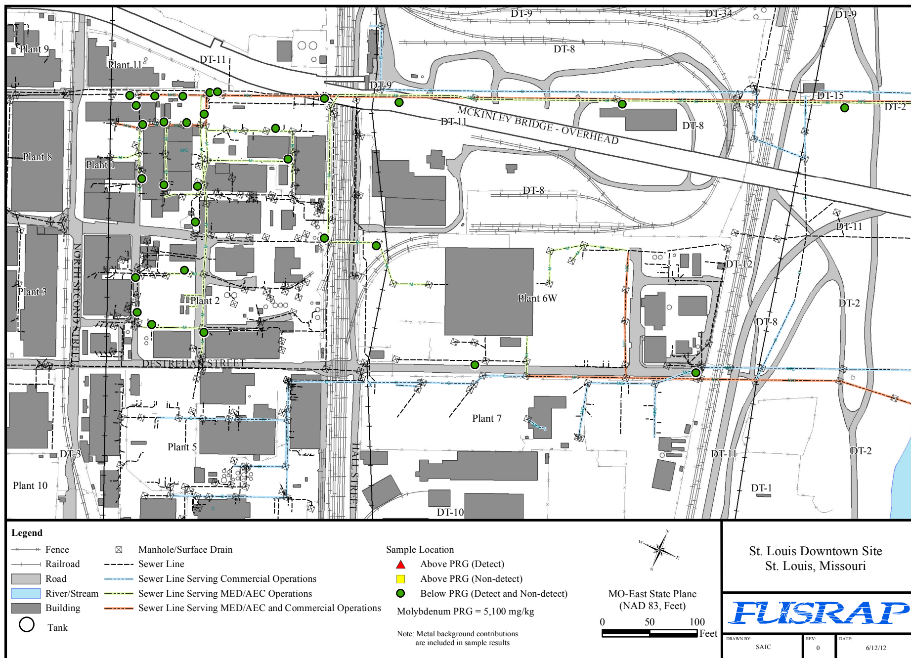
Figure H-37. Distribution of Molybdenum Exceeding the PRG in Soil Adjacent to Sewers
