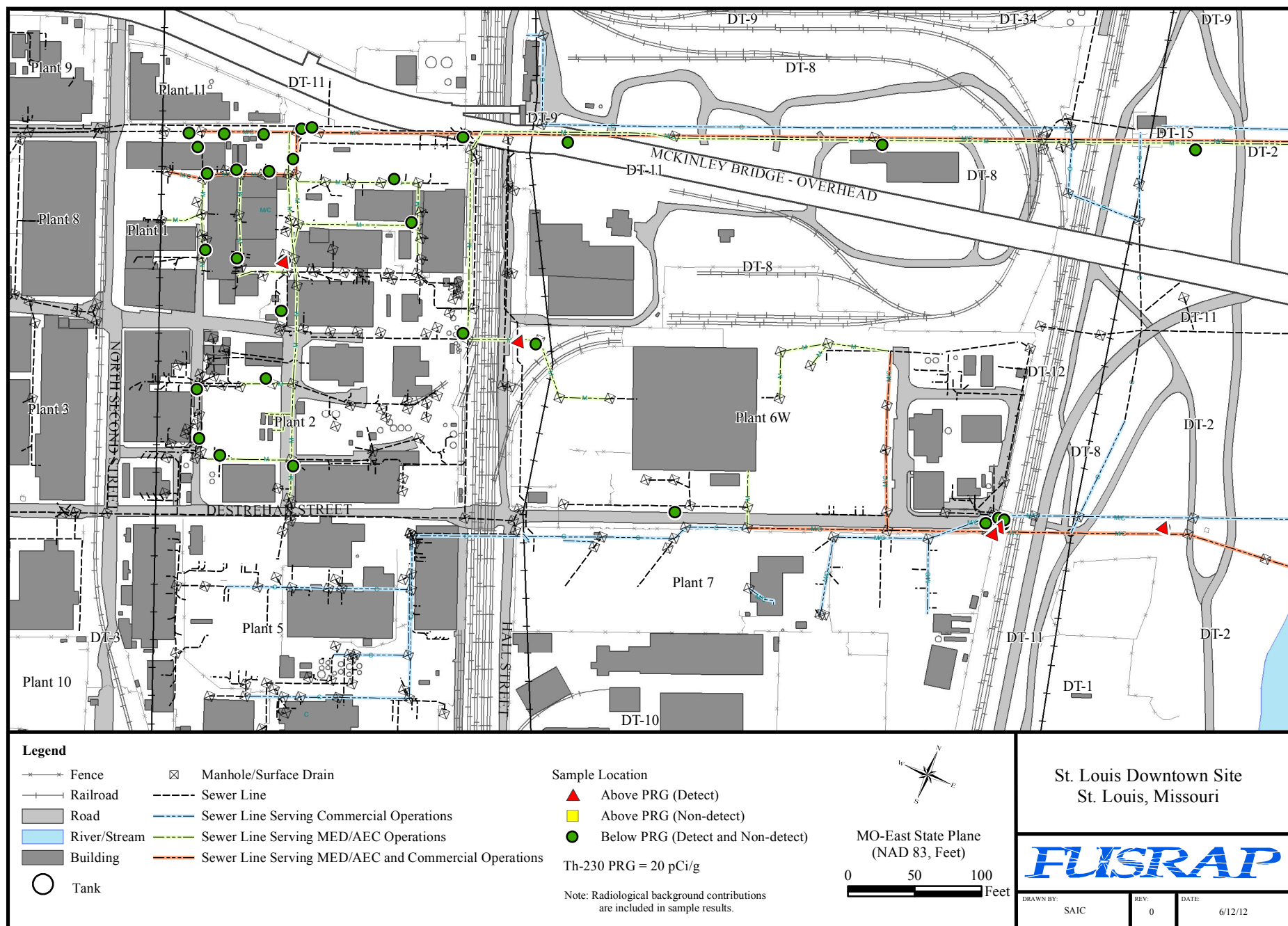
Figure H-27. Distribution of Th-230 Exceeding the PRG in Soil Adjacent to Sewers
