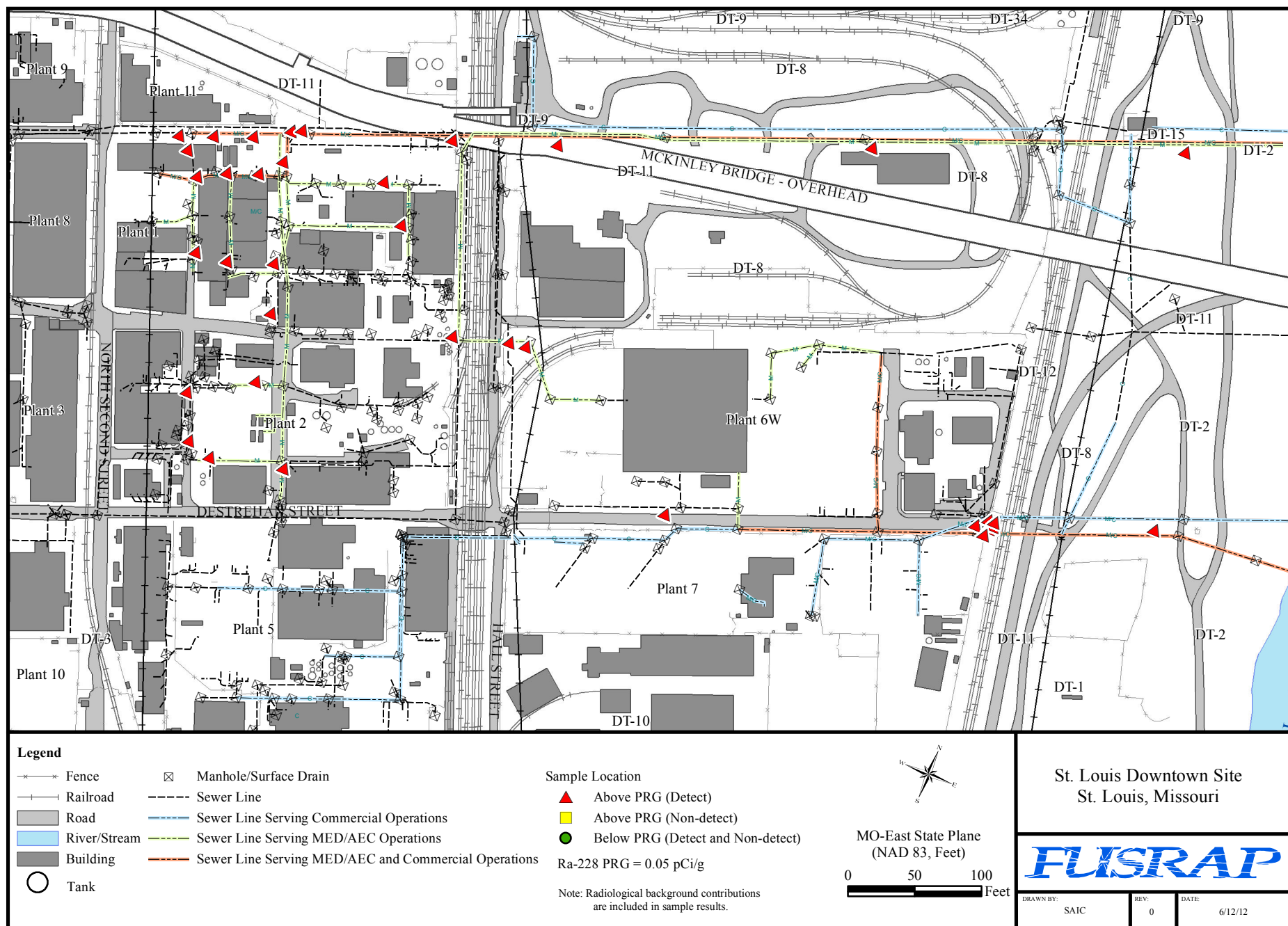
Figure H-25. Distribution of Ra-228 Exceeding the PRG in Soil Adjacent to Sewers
