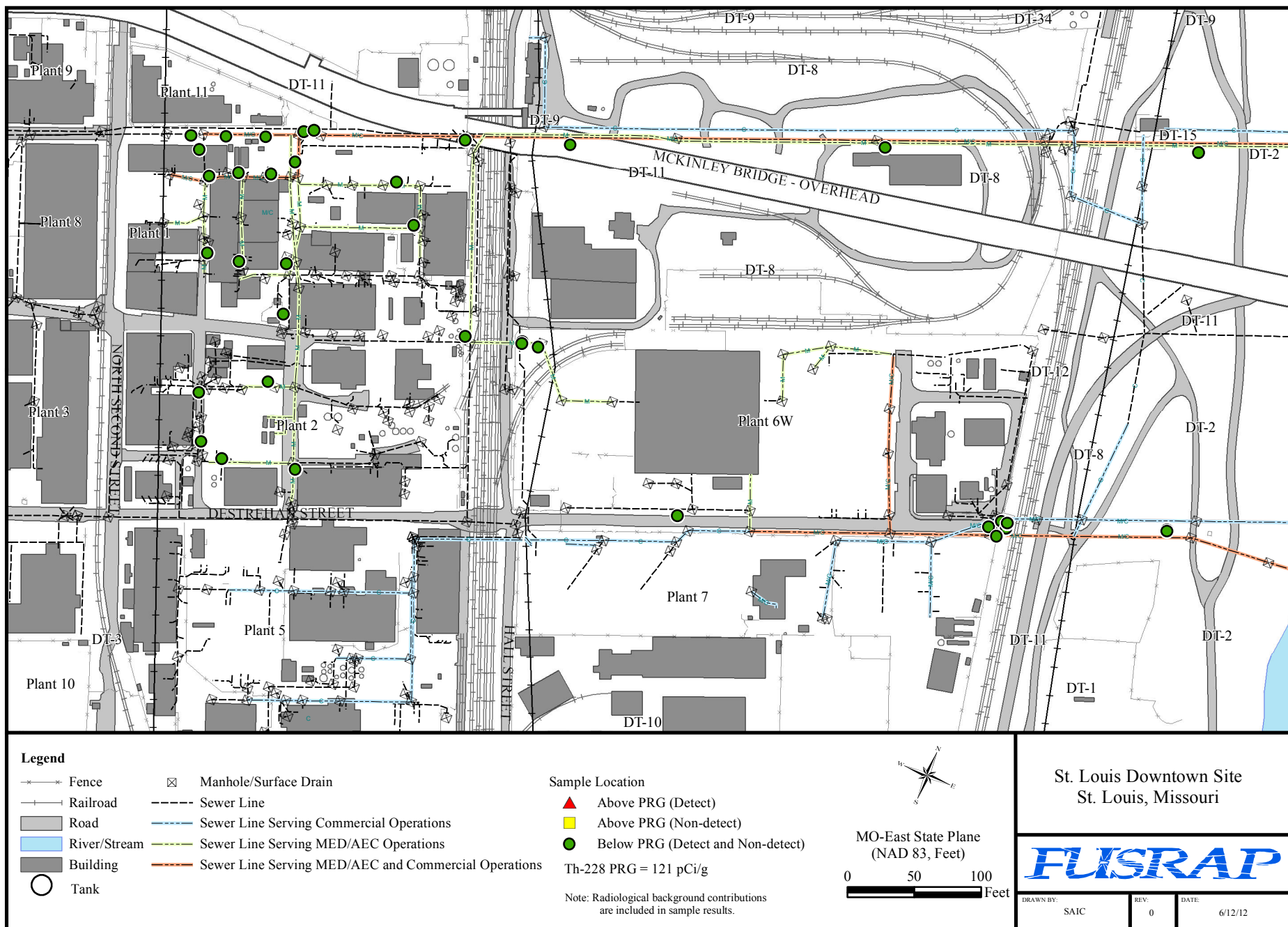
Figure H-26. Distribution of Th-228 Exceeding the PRG in Soil Adjacent to Sewers
