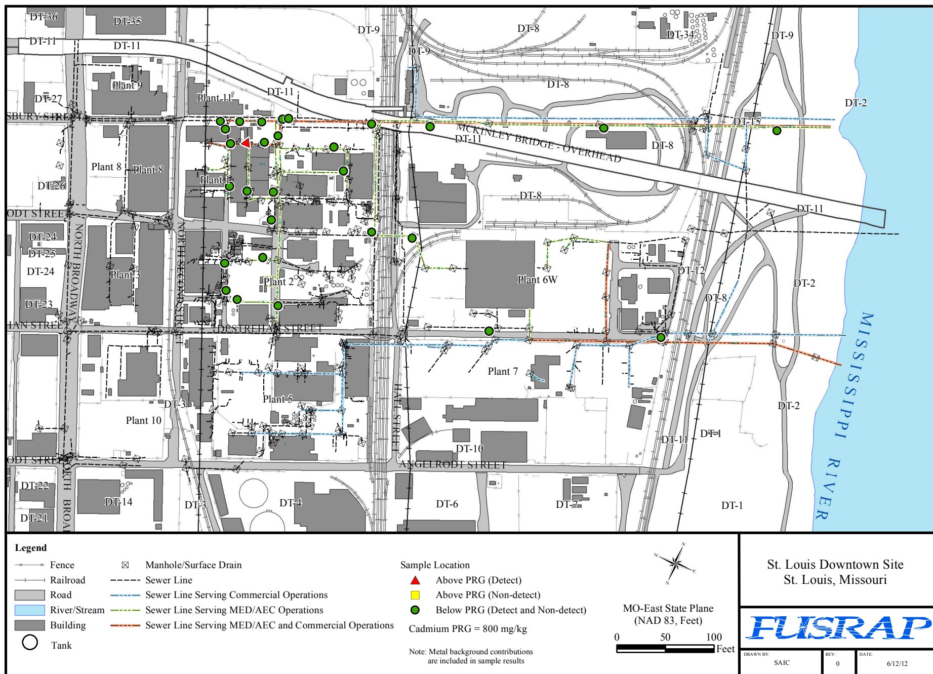
Figure H-32. Distribution of Cadmium Exceeding the PRG in Soil Adjacent to Sewers
