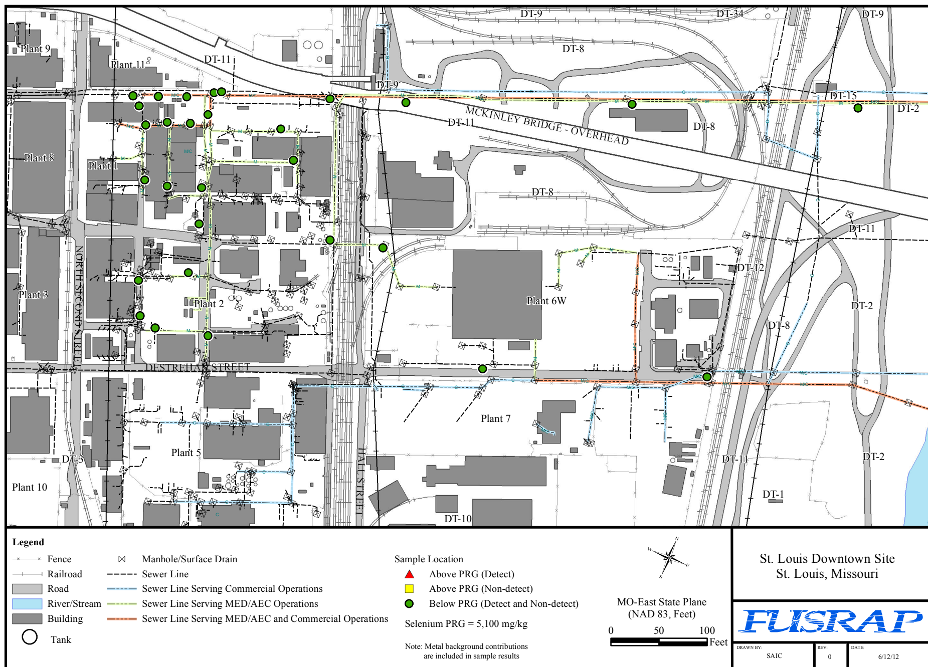
Figure H-39. Distribution of Selenium Exceeding the PRG in Soil Adjacent to Sewers
