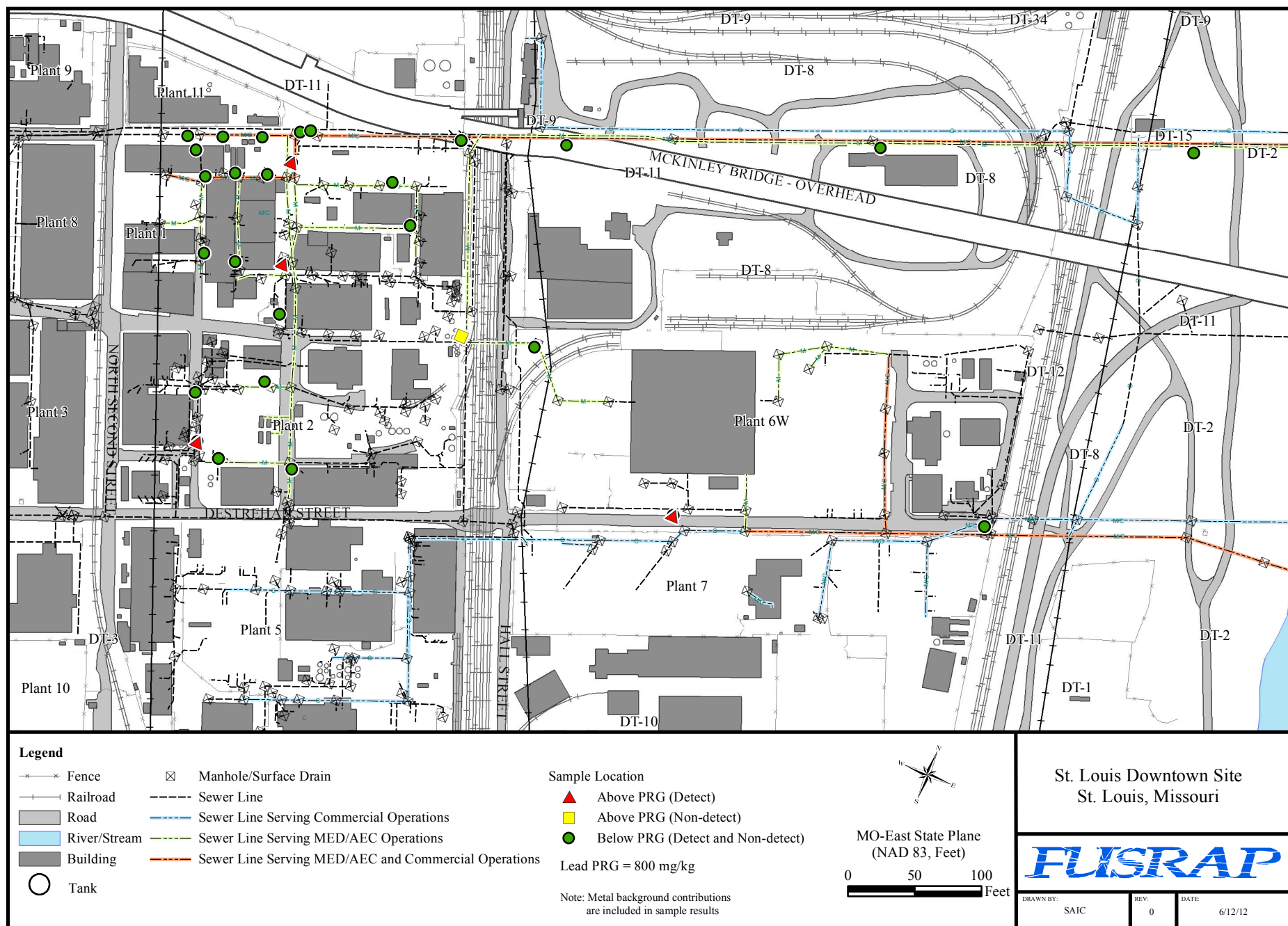
Figure H-35. Distribution of Lead Exceeding the PRG in Soil Adjacent to Sewers
